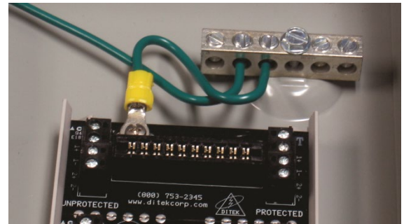
5-Position Grounding Buss in Use
